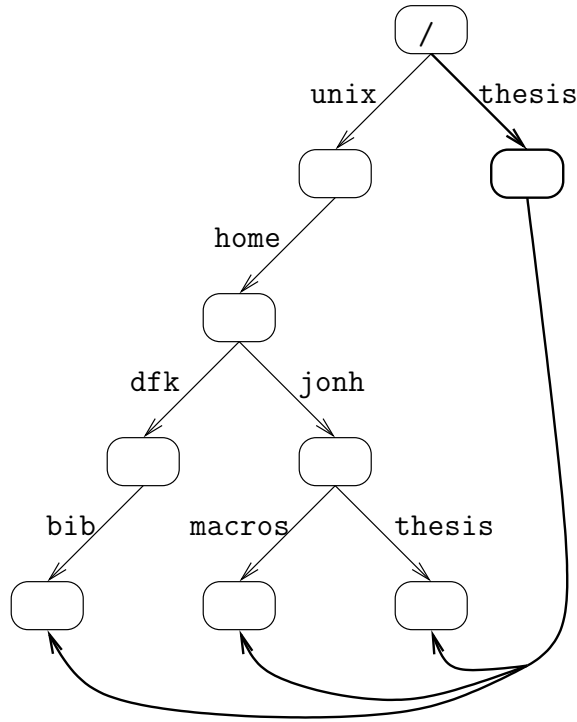
Figure 2.2: The same namespace can capture names at multiple levels of abstraction. In this Snowflake namespace, lower-level names (thin lines) embed location information, since they reflect location in a Unix file tree. The abstract name “/thesis” is implemented (thick lines) in terms of the lower level names, using a Union directory. Names at both levels of abstraction are Snowflake names.
