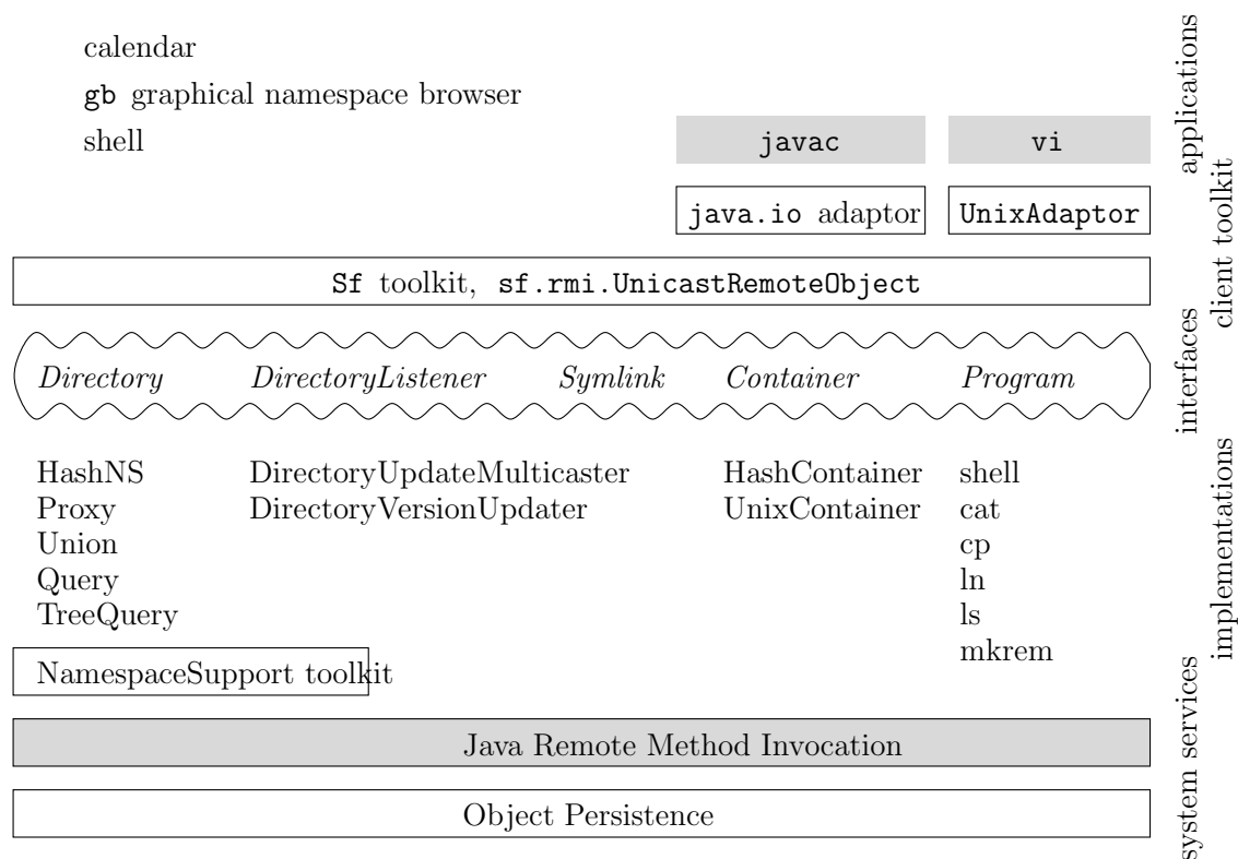
Figure 2.1: The layers of software that comprise the Snowflake naming implementation. The interfaces (in italics) determine the structure of the system; all name bindings are held in implementations of the Directory interface. Grey boxes indicate external components used in my environment.
