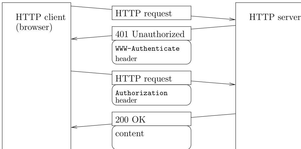
Figure 10.3: The HTTP authorization protocol.
