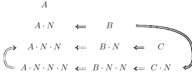
Figure 5.1: An example that shows when inherited names can become idempotent. Each arrow represents a speaks-for relationship; the text explains each arrow in more detail.
