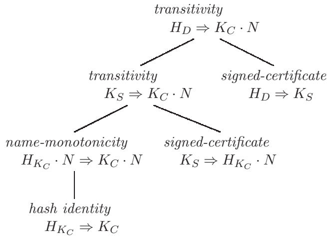
Figure 9.2: A structured proof that shows that a name defined by a client ( K_C \cdot N ) is bound to a particular document ( H_D ).
