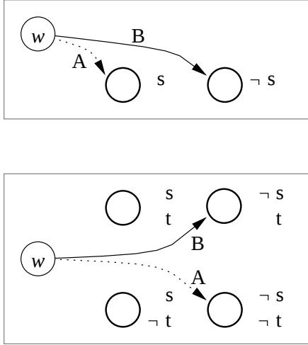
Figure A.6: Examples that show why the relation \xrightarrow{T} is weaker than \xRightarrow{T} and \xRightarrow{T} .
