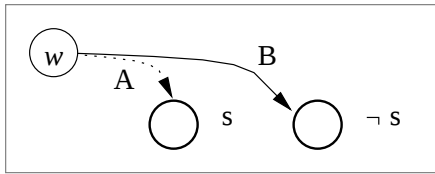
Figure A.4: A counterexample that shows B \xRightarrow{T} A does not imply B \xRightarrow{T} A .
