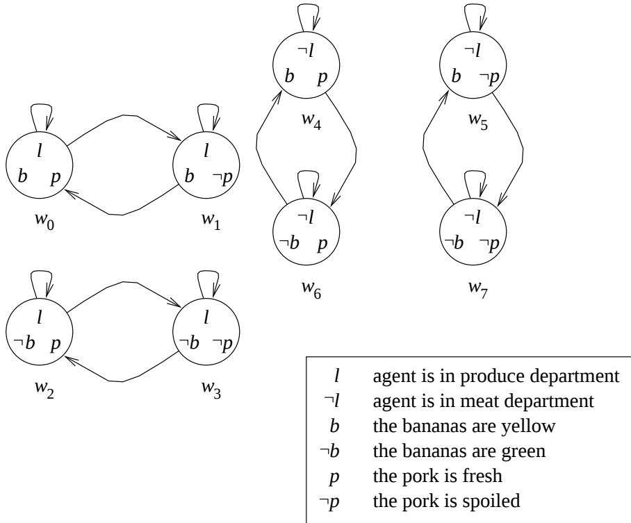
Figure B.1: A model of eight worlds (circles), illustrating the relationship between the accessibility relation (arrows) and the modal operator ( A believes ).
